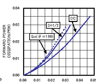
AVERAGE RECTIFIED FORWARD CURRENT Io(A) Io-Pf CHARACTERISTICS
