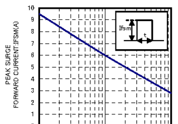
IFSM-t CHARACTERISTICS
