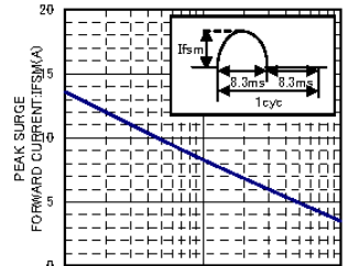
IFSM-CYCLE CHARACTERISTICS
